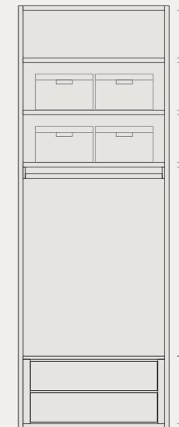
3 ripiani 1 tubo appendiabiti 1 cassettiera interna con 2 cassetti 3 shelves 1 coat-hanger 1 inner drawer with 2 drawers
